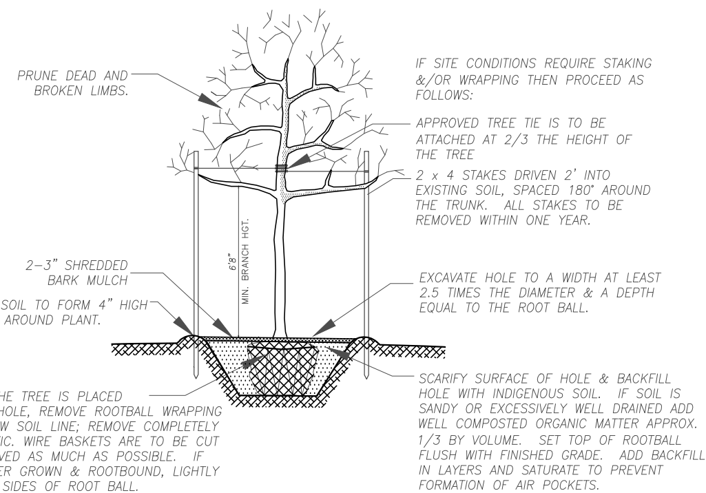
TREE PLANTING DETAIL SCALE: NONE
