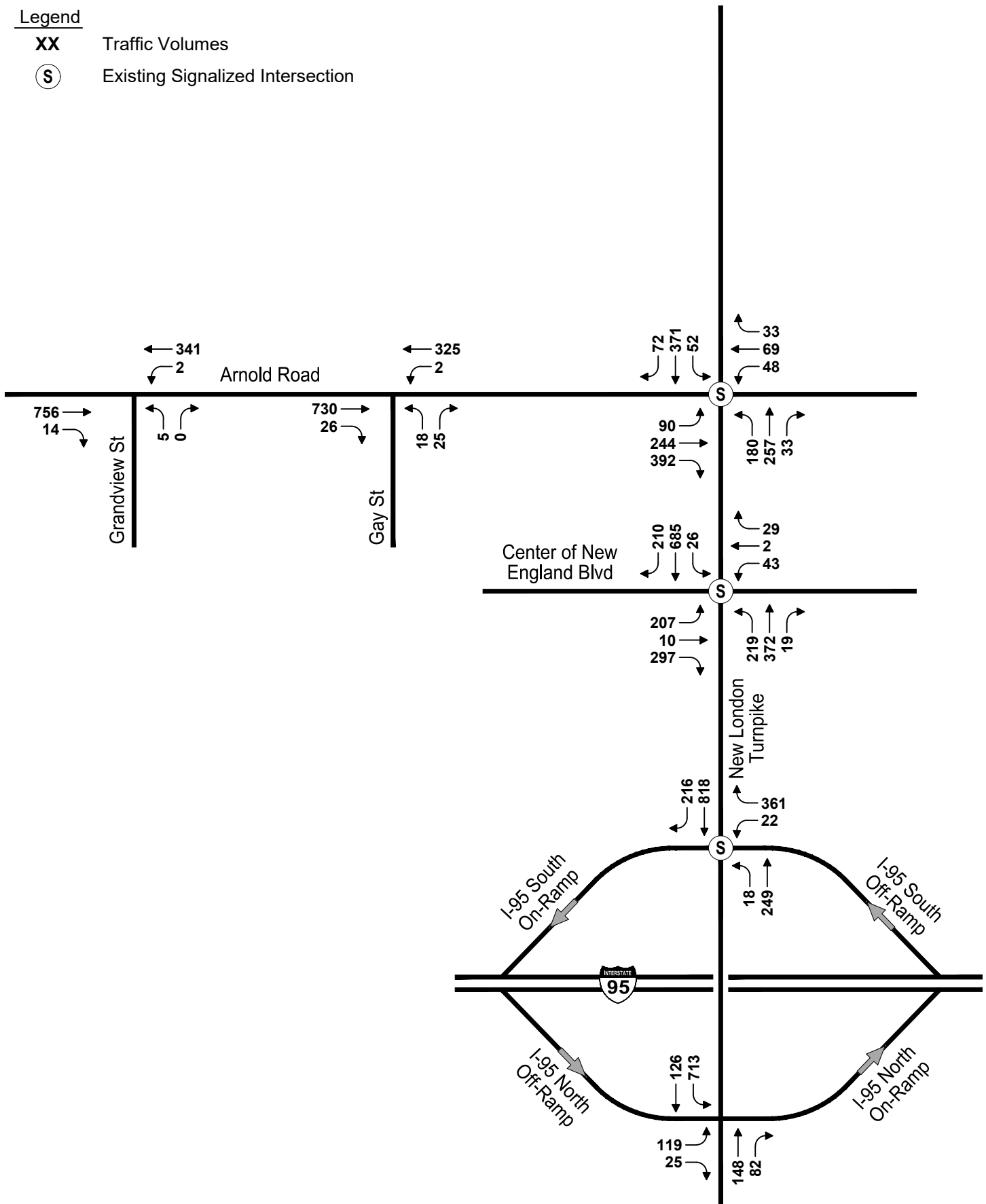
2030 No-Build Weekday Morning Peak Hour Traffic Volumes New London Turnpike at Arnold Road Coventry, RI
