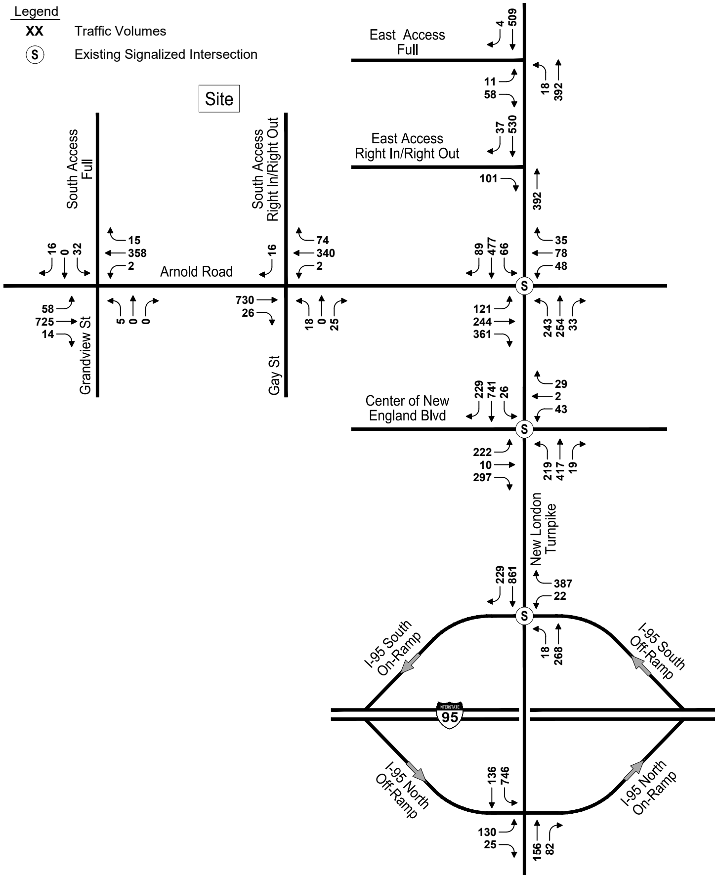
2030 Build Weekday Morning Peak Hour Traffic Volumes New London Turnpike at Arnold Road Coventry, RI
