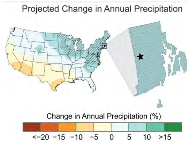
Figure 12- Rhode Island Projected Change in Annual Precipitation
