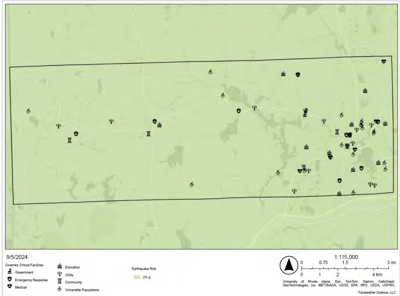
Figure 34- Coventry Earthquake Risk Map
