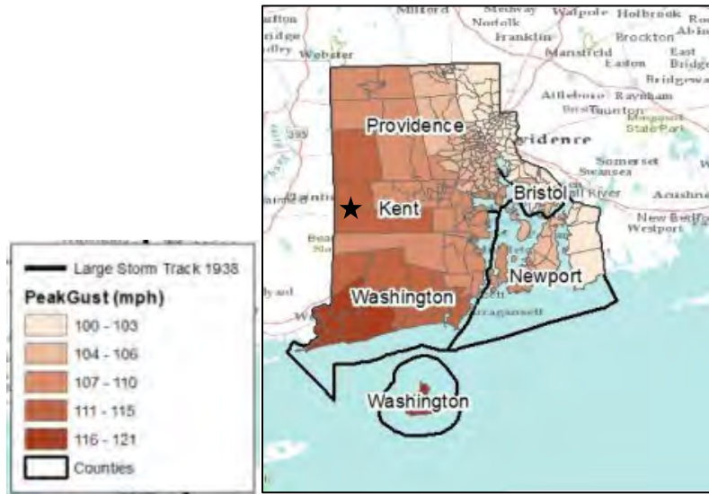
Figure 16- Peak Wind Gust of the 1938 Great Hurricane
